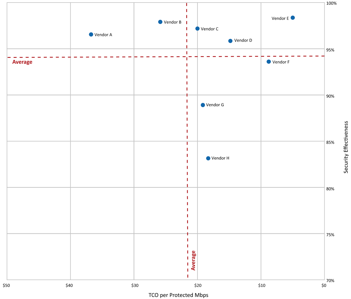
Figure 3 – Example SVM
